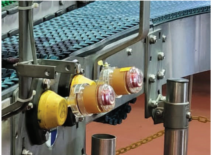
LubeSite - Single Point Lubricator
