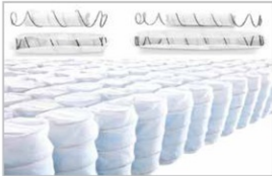
NESTED POCKETED SPRINGS WIRE DIAMETER : 1.9 ~ 2.1 MM
